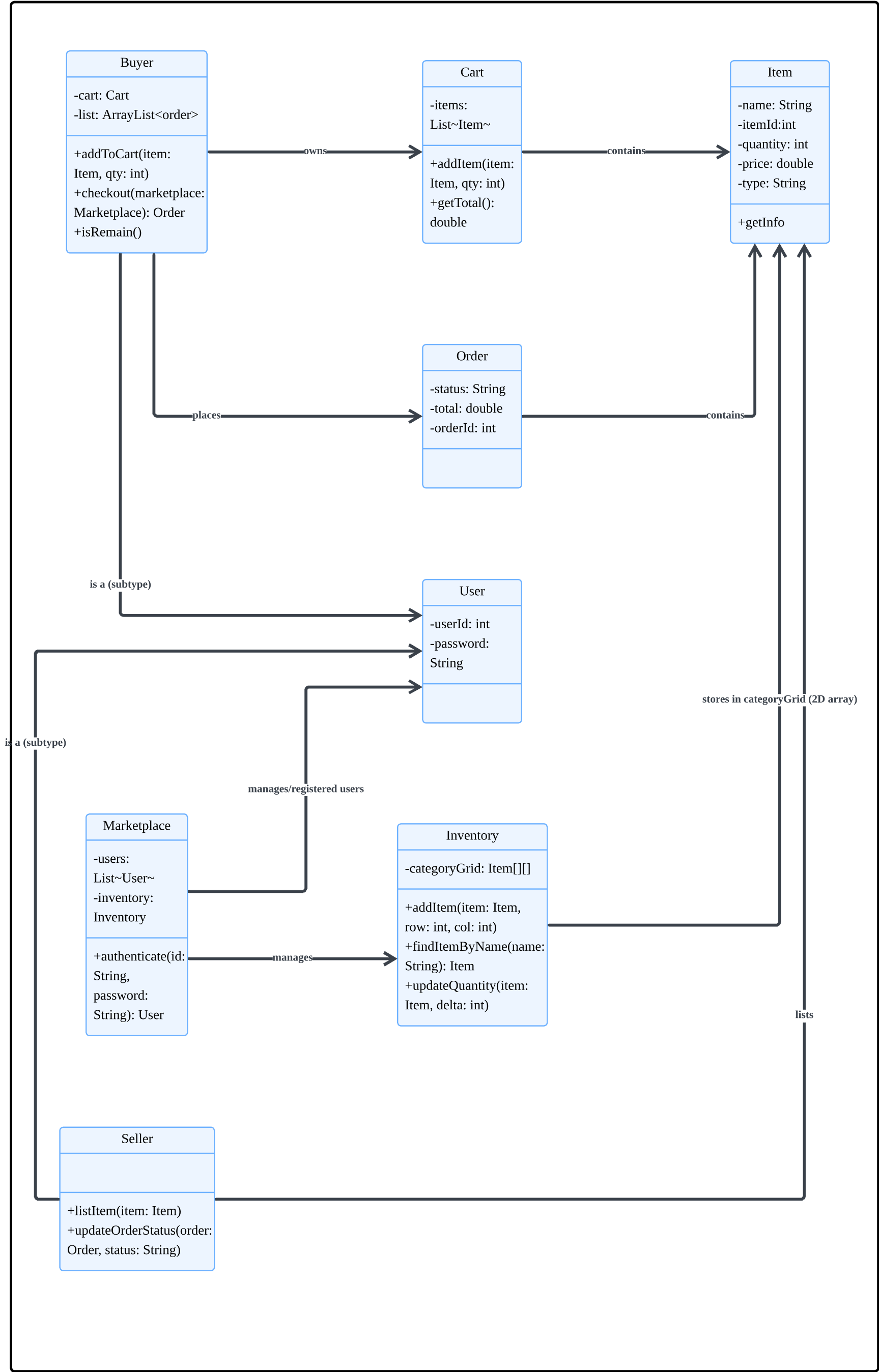
LoveCube Marketplace: Simplified Class Diagram
